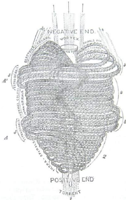
Fig. 135. The general Form of an Atom, including the spirals and 1st Spills, together with influx and efflux ethers, represented by dots, which pass through these spirilla. The 2d and 3d spirilla with their still finer ethers are not shown.
